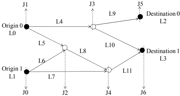
Fig. 3. Traffic network
