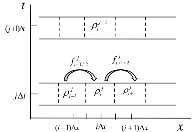
Fig. 1. Godunov method for the LWR model
